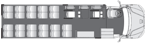
22 Passenger 2 Wheelchair with Foldaway Seats Plus Driver
