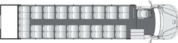
37 Passenger with Rear Luggage Plus Driver
