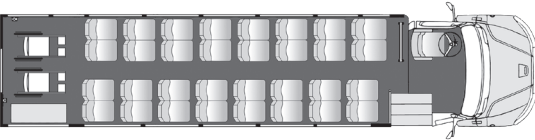
32 Passenger 2 Wheelchair Plus Driver
