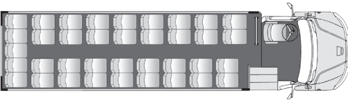
37 Passenger Plus Driver
