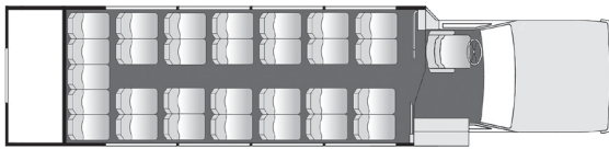
29 Passenger with Rear Luggage Plus Driver
