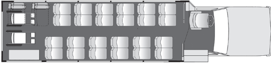
24 Passenger 2 Wheelchair with Foldaway Seats Plus Driver
